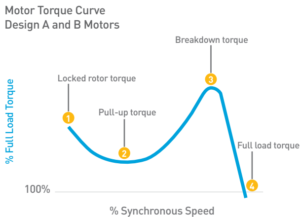
Figure 3: Design A and B Motor Torque Curve
