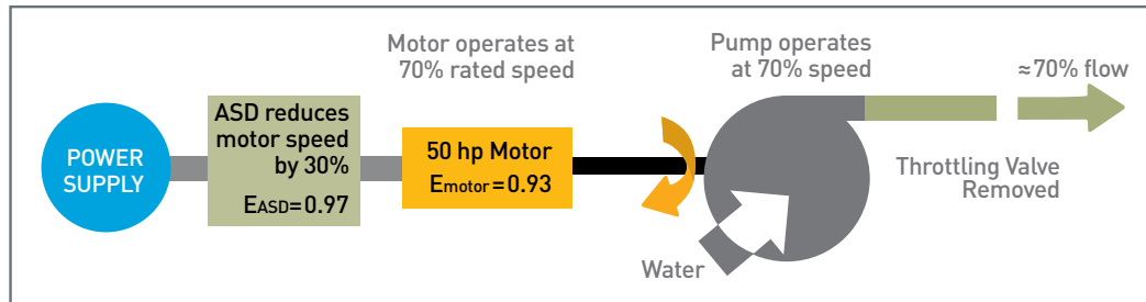
Figure 6: Pump System Diagram with ASD
