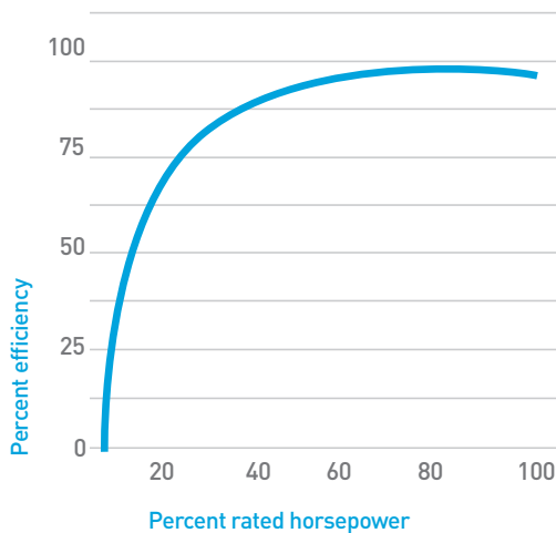
Figure 4: Efficiency versus Load Curve for Induction Motors
