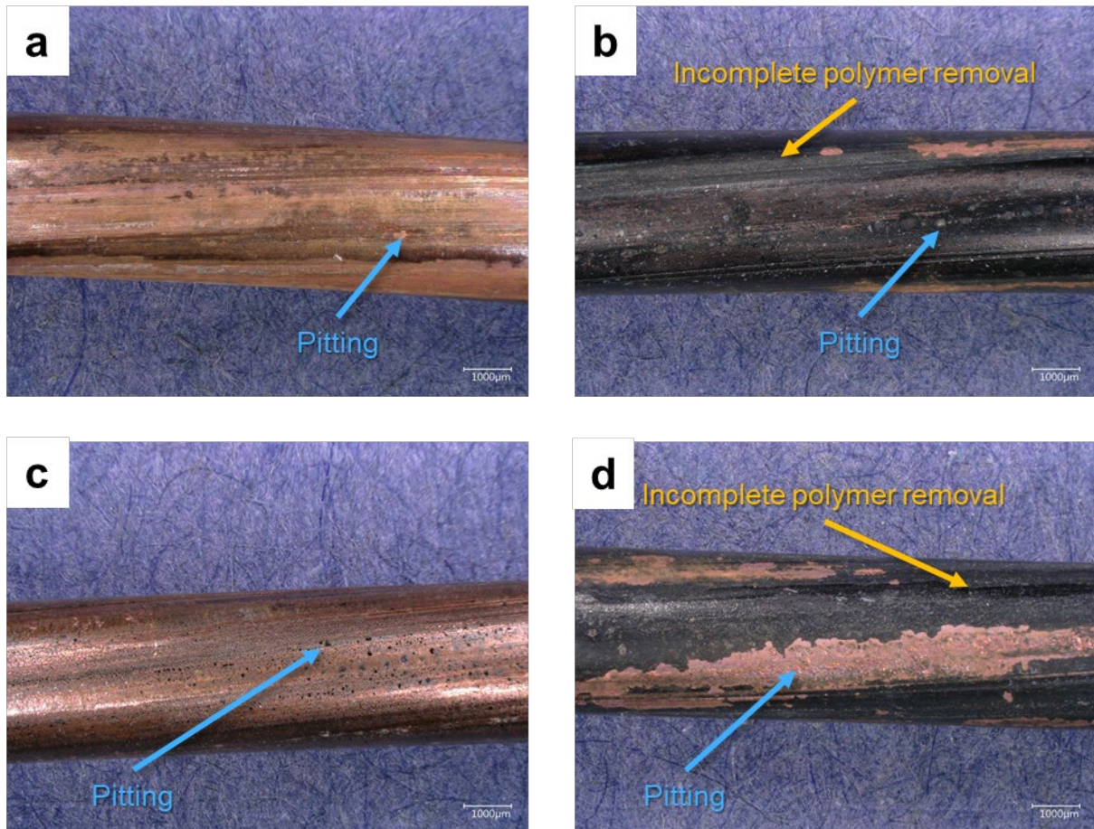
Figure 40. Representative optical microscopy images of core strands from a salt-spray-tested (a) bare 17-kV copper conductor, (b) Ripley-stripped 17-kV copper CC, (c) manually stripped 17-kV copper CC, and (d) 17-kV copper CC with midspan damage. The areas in (b-d) were underneath the polymer sheath during salt spray testing.
