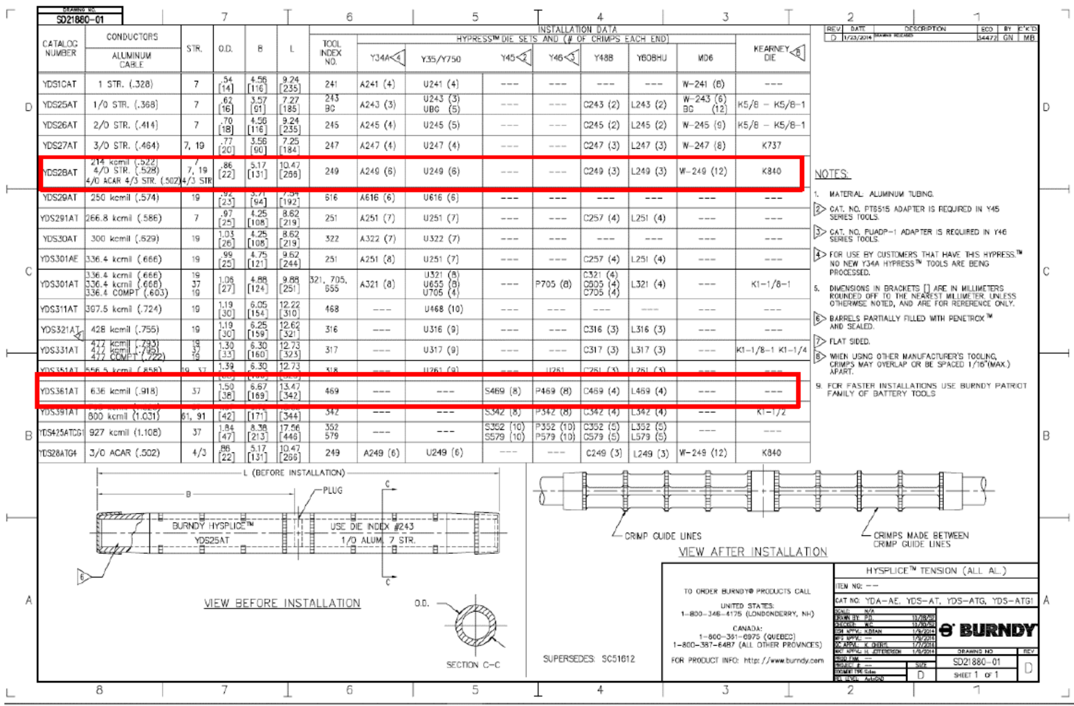
Figure B - 5: Burndy Drawing for HYSPLICE™ - YDS311AT
