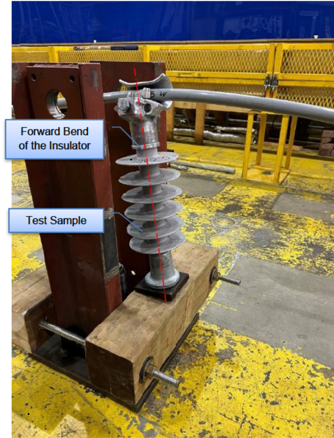
Figure 6-9: K-Line KL46SK - Typical Clamp and 1/0 AWG ACSR (35 kV) Conductor Position after Slip Test
