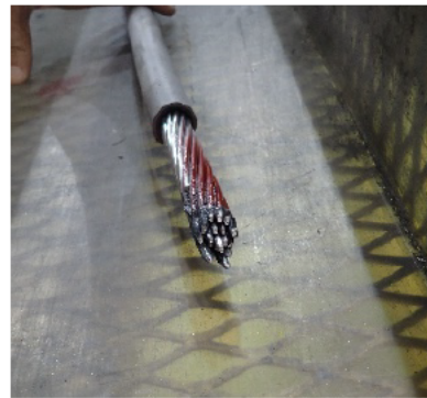
Figure 6-12: Sample 1.3.2 after test
