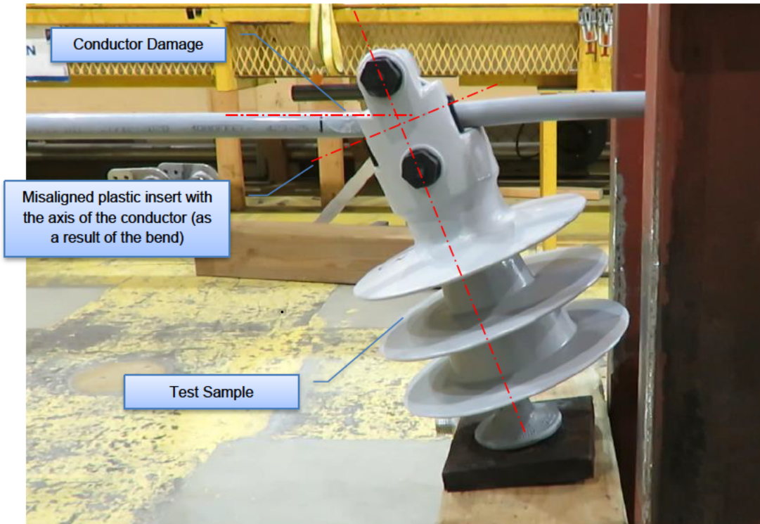
Figure 6-1: Hendrix HPI-35VTP-02 - Typical Clamp and 1/0 AWG (17 kV) ACSR Conductor Position after Slip Test
