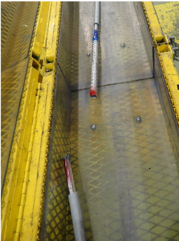
Figure 6-12: Sample 1.3.2 after test
