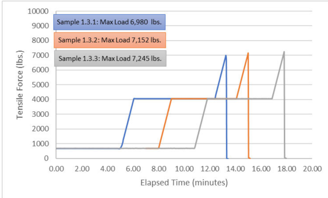
Figure 6-3: Maximum Load Test – 22 kV, 397.5 kcmil AAC
