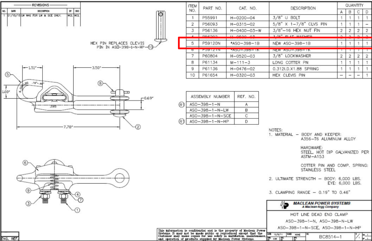
Figure 8-2: MPS Dead-End Bolted Clamp ASO 398
