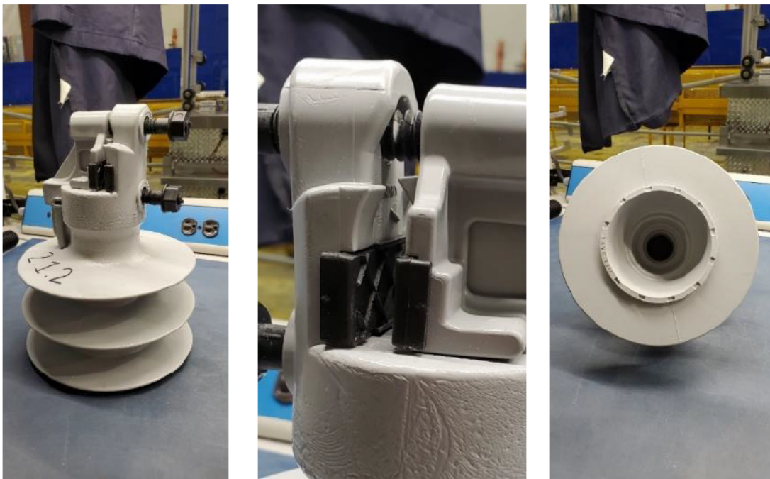
Figure 6-6: Hendrix HPI-35VTP-02 - Typical Insulator Condition after Slip Test (no damage)
