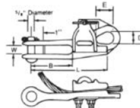
ONE "U" BOLT ADSO
