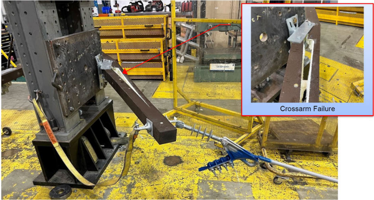
Figure E4. A representative post-test image showing splitting and failure of the composite cross-arm. 336.4 kcmil ACSR (30/7) with ADE-23 dead-end shown.
