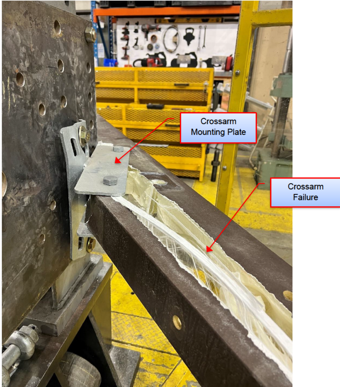
Figure 6-20: Sample 5.1 – Failure Location
