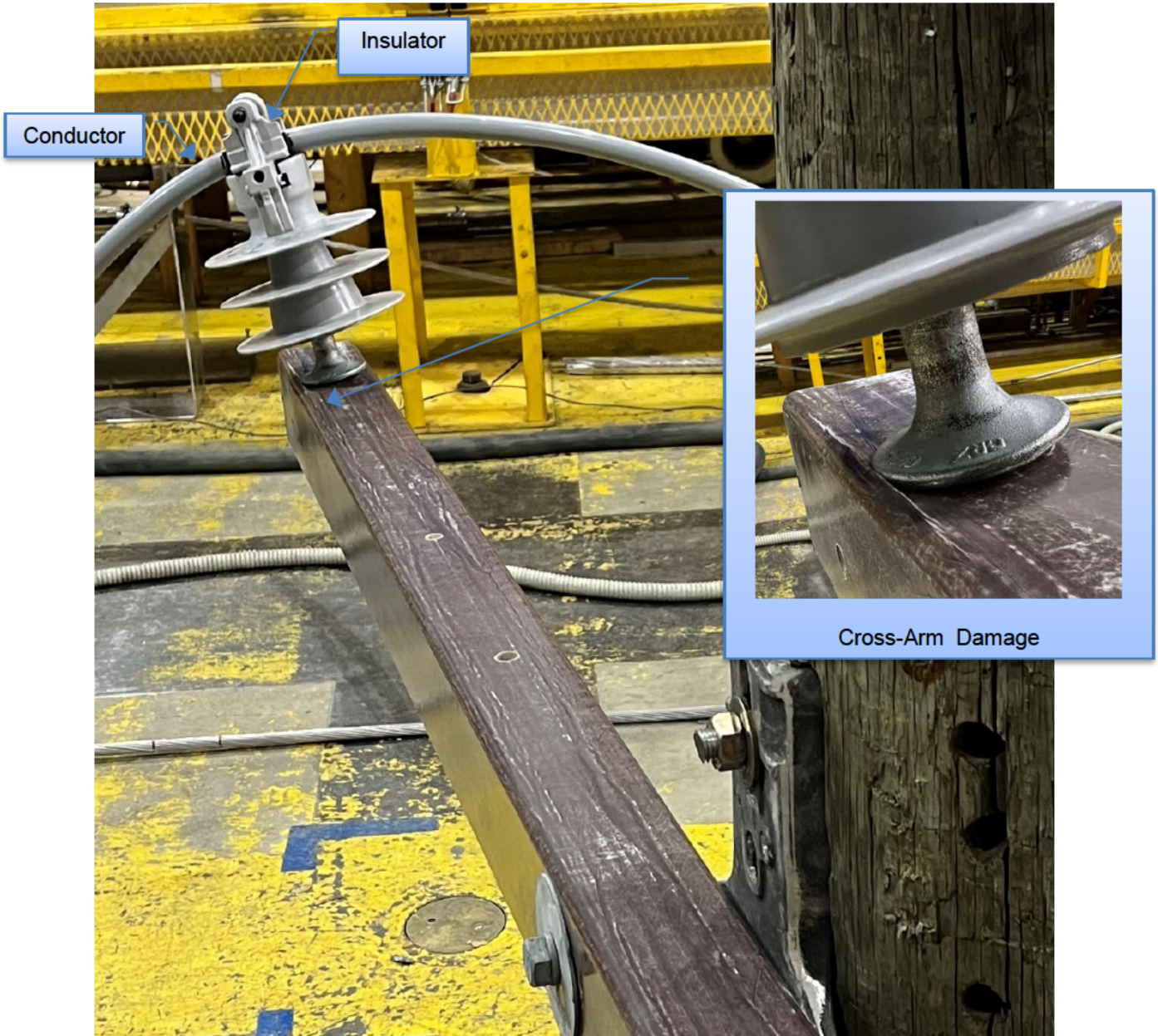
Figure 6-13: Sample 3.2.1 – Insulator and Cross-arm Condition after Test
