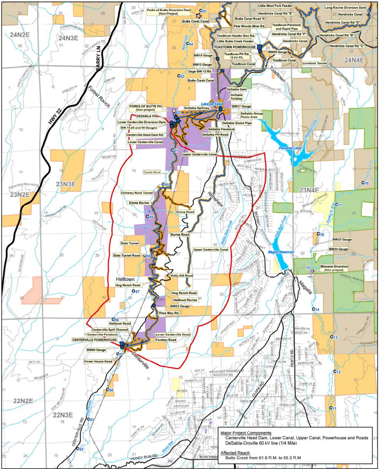
Desabla-Centerville Project FERC 803 © 2004, PACIFIC GAS AND ELECTRIC CO. Figure E6.3.2-6-1a Middle Butte Subreach Lower Butte Instream Flow Study Area Centerville Canals and Powerhouses
