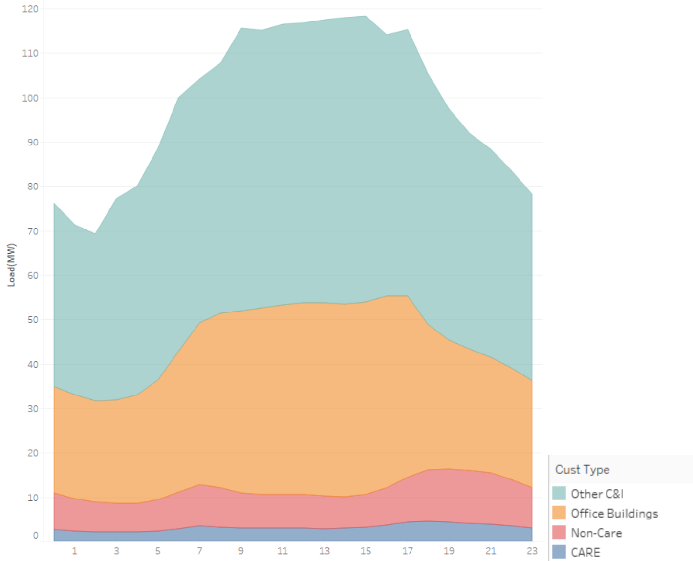
Winter Peak Load Day - December 2015
