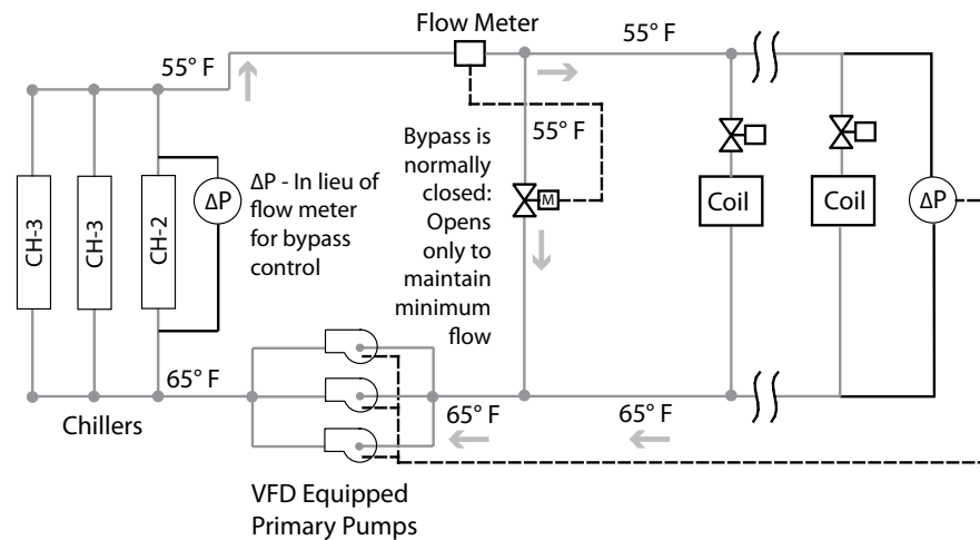
Figure 5.03: Primary only Chilled Water Pumping Schematic (Source: Created by Integral Group)
