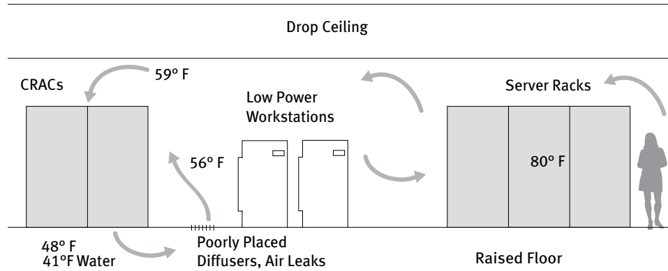
Figure 2.02: Poor airflow Conditions (Source: Created by Integral Group)
