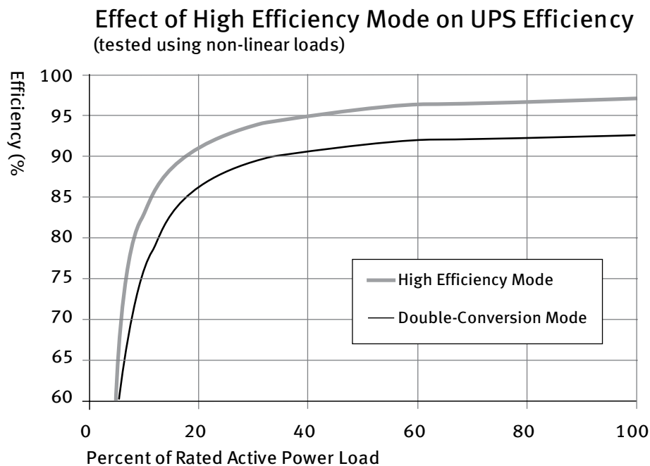
Figure 10.05: Effect of High Efficient Mode 3
