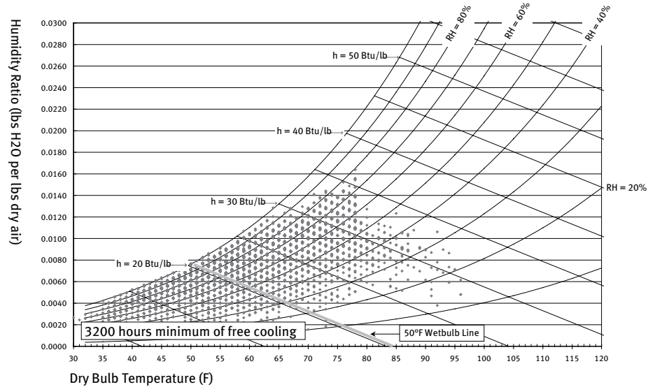
Figure 7.03: Psychrometric chart for San Jose, California (Source: Created by Integral Group)
