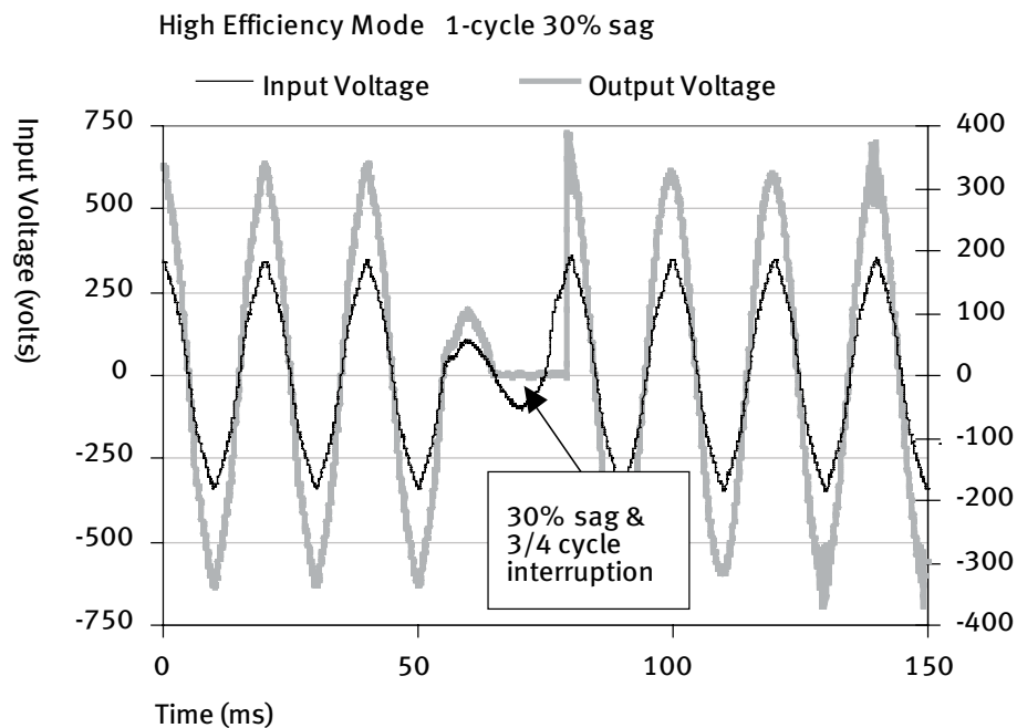
Figure 10.06: Interruption of Power when switching from passive standby mode to high efficiency mode 3
