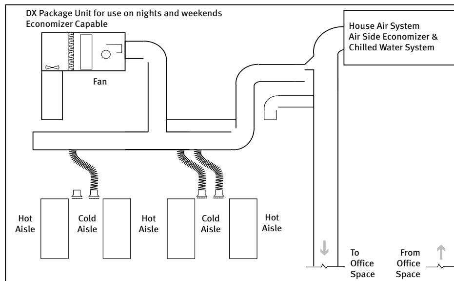
Figure 3.03 : Schematic Diagram of Air Distribution System (Source: Created by Integral Group)
