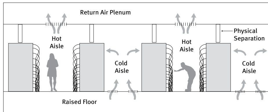
Figure 2.01: Hot Aisle/Cold Aisle Arrangement
