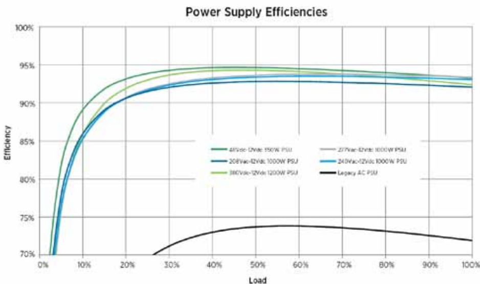
Figure 1.01: Efficiencies at varying load levels for typical power supplies (Source: Quantitative Efficiency Analysis of Power Distribution Configurations for Data centers, The Green Grid)
