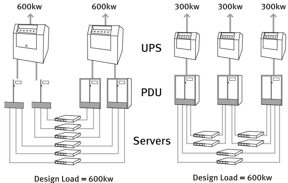
Figure 10.03: An efficiency gain is realized when operating smaller UPS systems at partial loads as opposed to larger systems as partial loads 1
