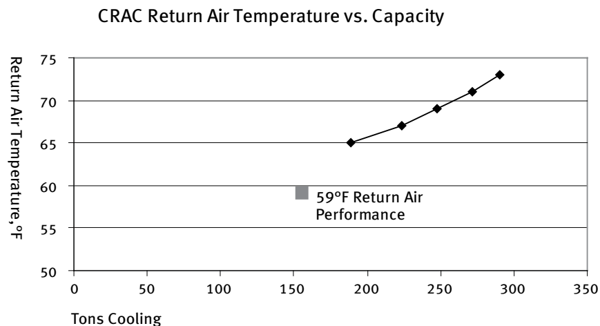
Figure 2.03: CRAC Return Air Temperature vs Capacity (Source: Created by Integral Group)
