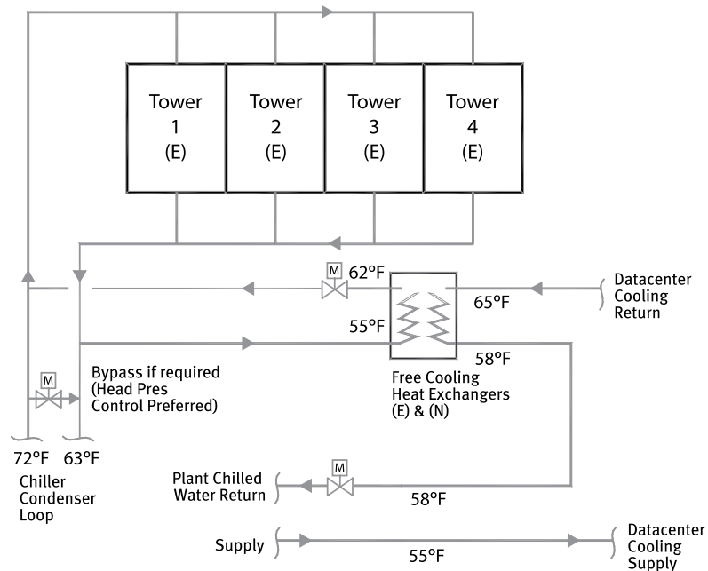
Figure 7.02: Free Cooling Loop Schematic
