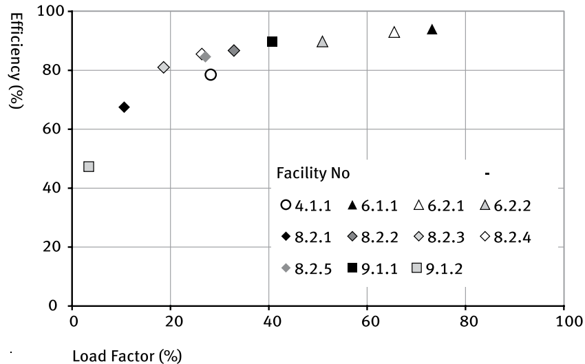
Figure 10.04: Measured Efficiencies of UPS Systems 2
