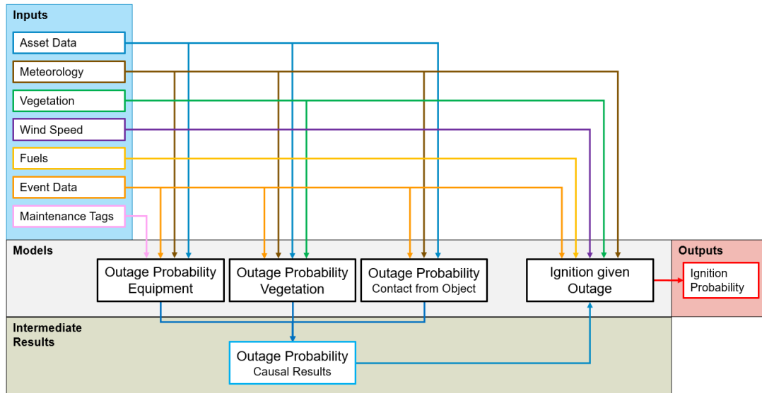
FIGURE-5-2-1: DISTRIBUTION IGNITION LIKELIHOOD CALCULATION SCHEMATIC
