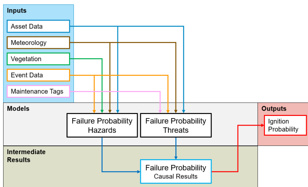
FIGURE 5-2-2: TRANSMISSION IGNITION LIKELIHOOD CALCULATION SCHEMATIC
