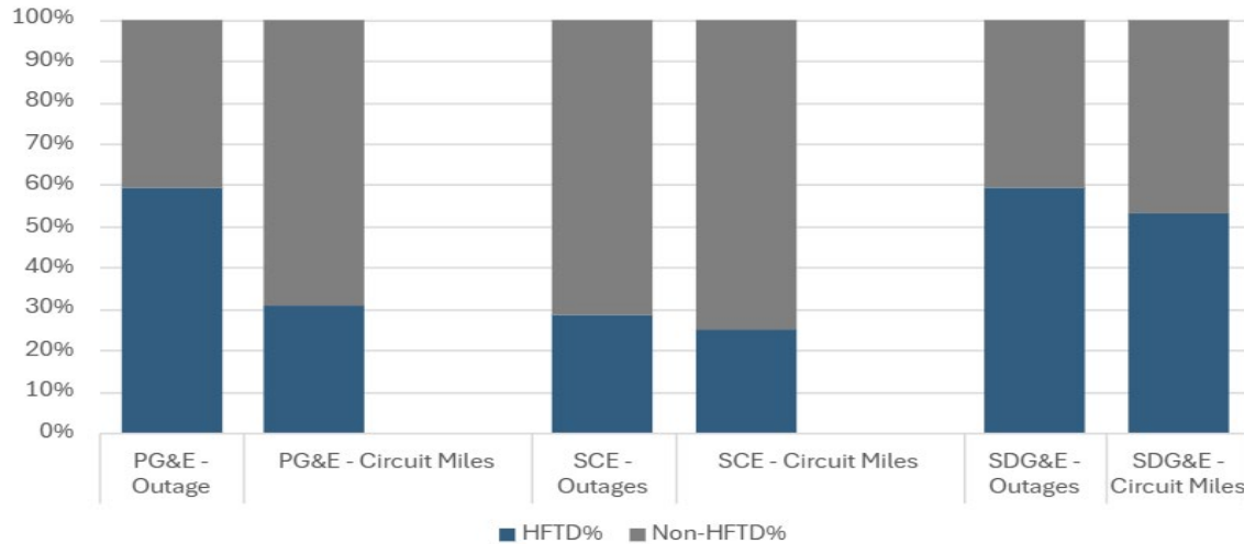
Figure 3: Comparison of Vegetation Caused Outages During RFW Conditions that do not Trigger PSPS Protocols
