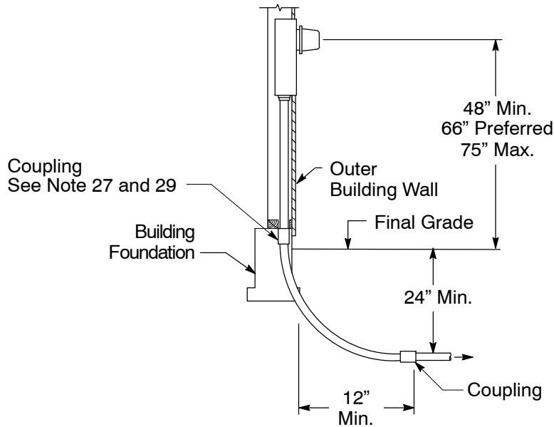
Figure 2 Recessed-Mounted Service Termination Enclosure
