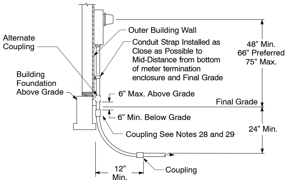
Figure 3 Surface-Mounted Service Termination Enclosure
