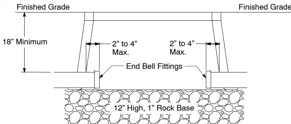
Figure 1 Conduit Installation in a Drain Box
