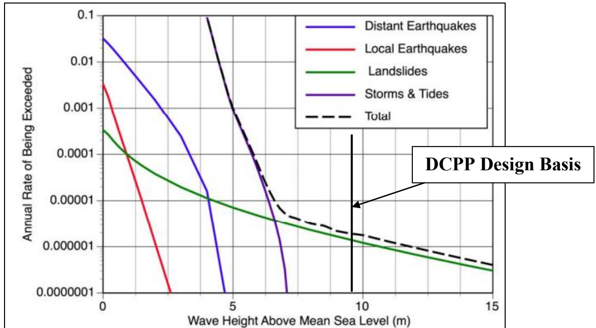
Mean hazard from storms, tides, and tsunamis for the DCPD intake structure
