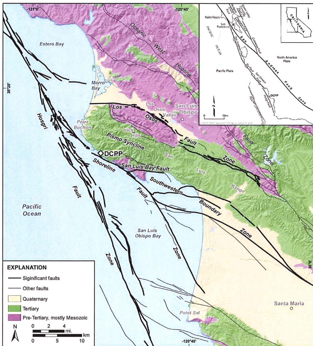
Figure 2.0-1: Simplified Geology and Faults in DCP's Vicinity
