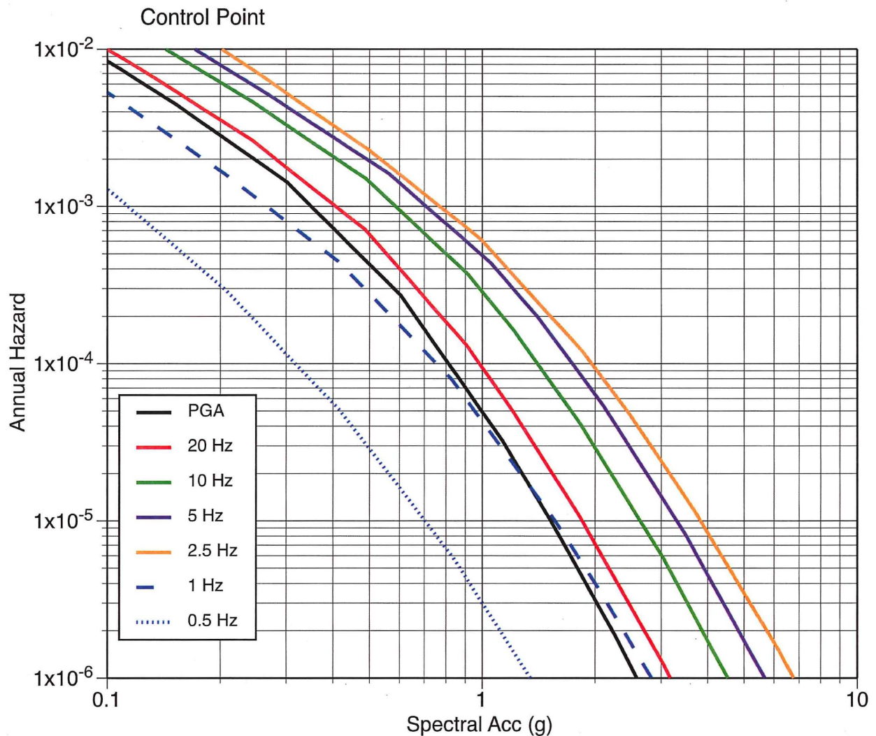
Figure 2.3.7-1 Control Point Mean Hazard Curves for PGA and 20, 10, 5, 2.5, 1, and 0.5 Hz Spectral Frequencies
