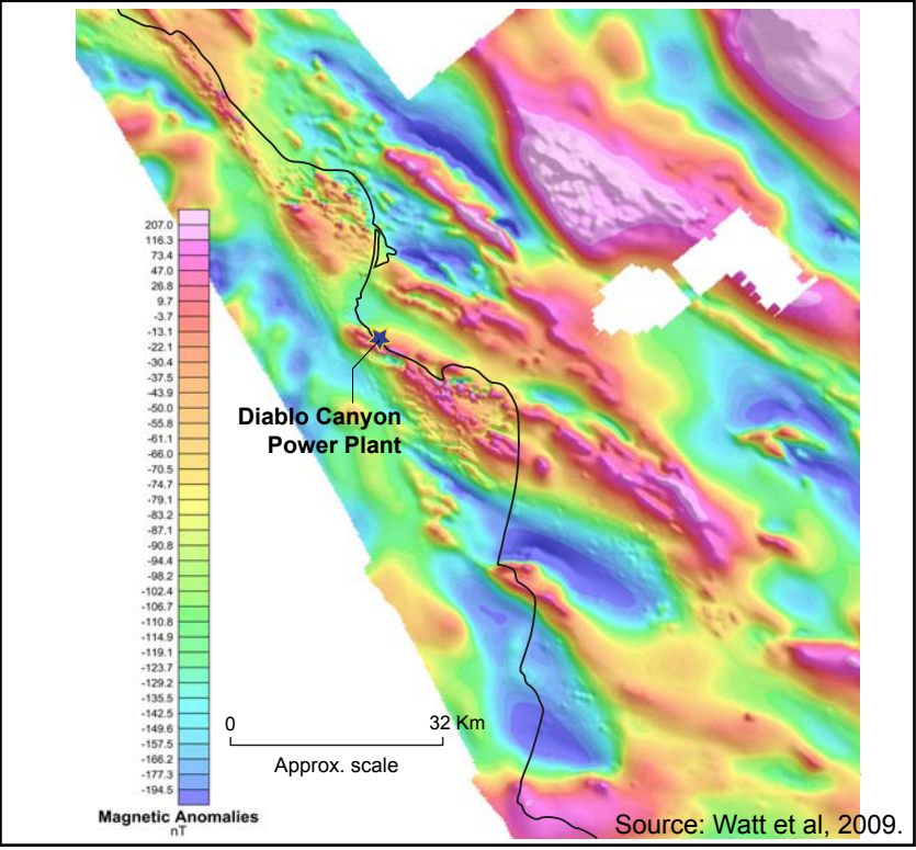
c. Regional Magnetic Anomalies
