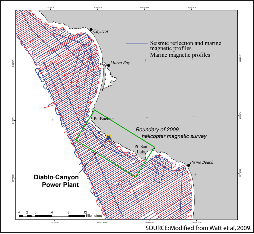
b. New Marine Geophysical Data Collected in 2008-2009
