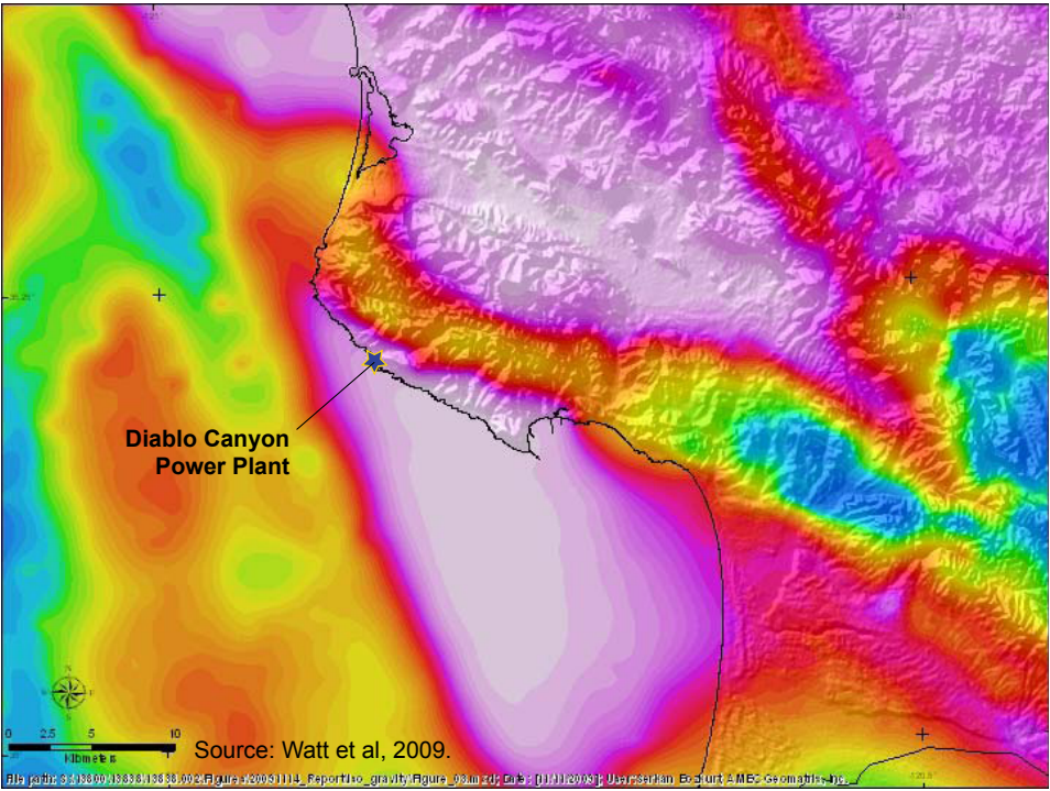
d. Regional Isostatic Gravity Anomalies
