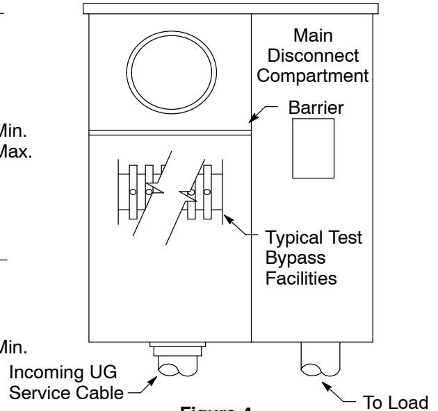
Figure 4 Typical Service Termination Enclosure for Non-Residential 3-Wire or 4-Wire Service 0–200 Amp Maximum 0–600 V (see Note 6 on Page 3) (see Figure 2 on Page 3 for typical residential enclosure)
