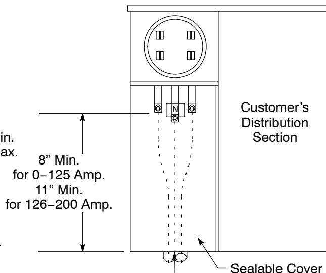
Figure 2 Typical Residential Combination Service Termination Enclosure and Meter Socket Panel, 200 Amp Max., 120/240 V
