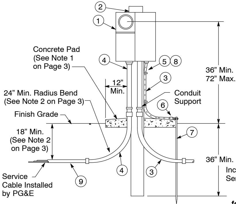
Figure 3 Non-Residential Service (or residential service installed in conduit)
