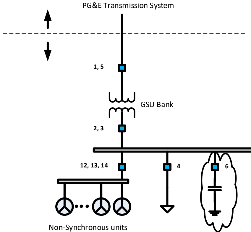
Figure 2.1-B - Example Non-Synchronous Generator Telemeter Points
