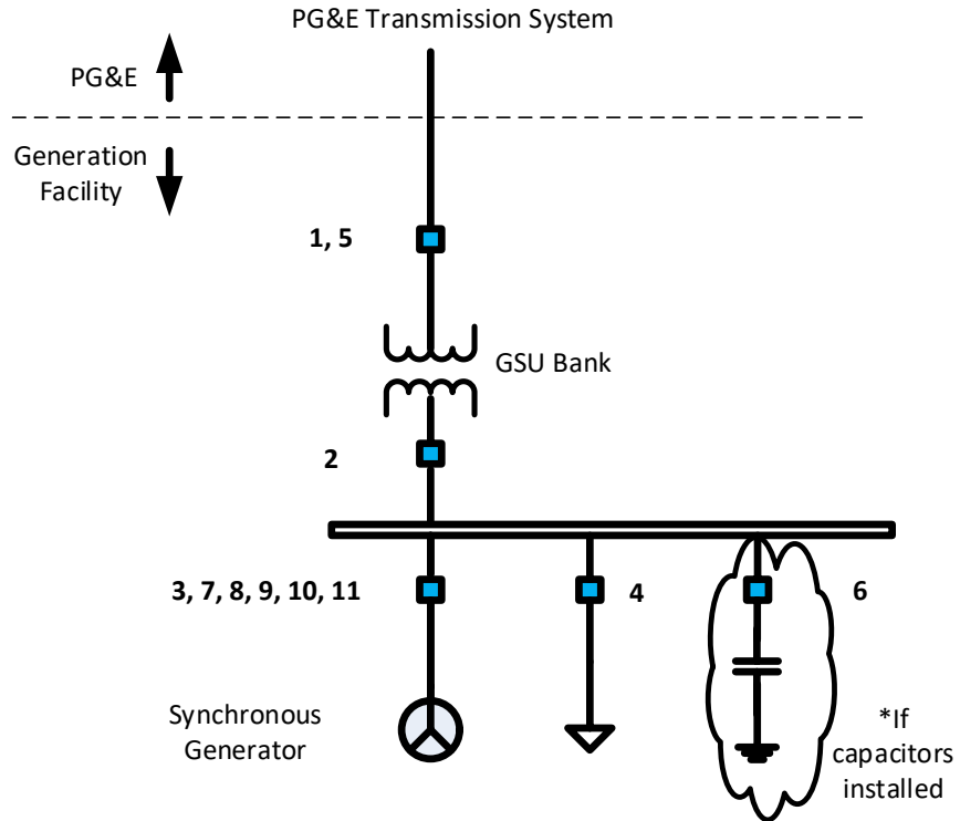
Figure 2.1-A - Example Synchronous Generator Telemeter Points
