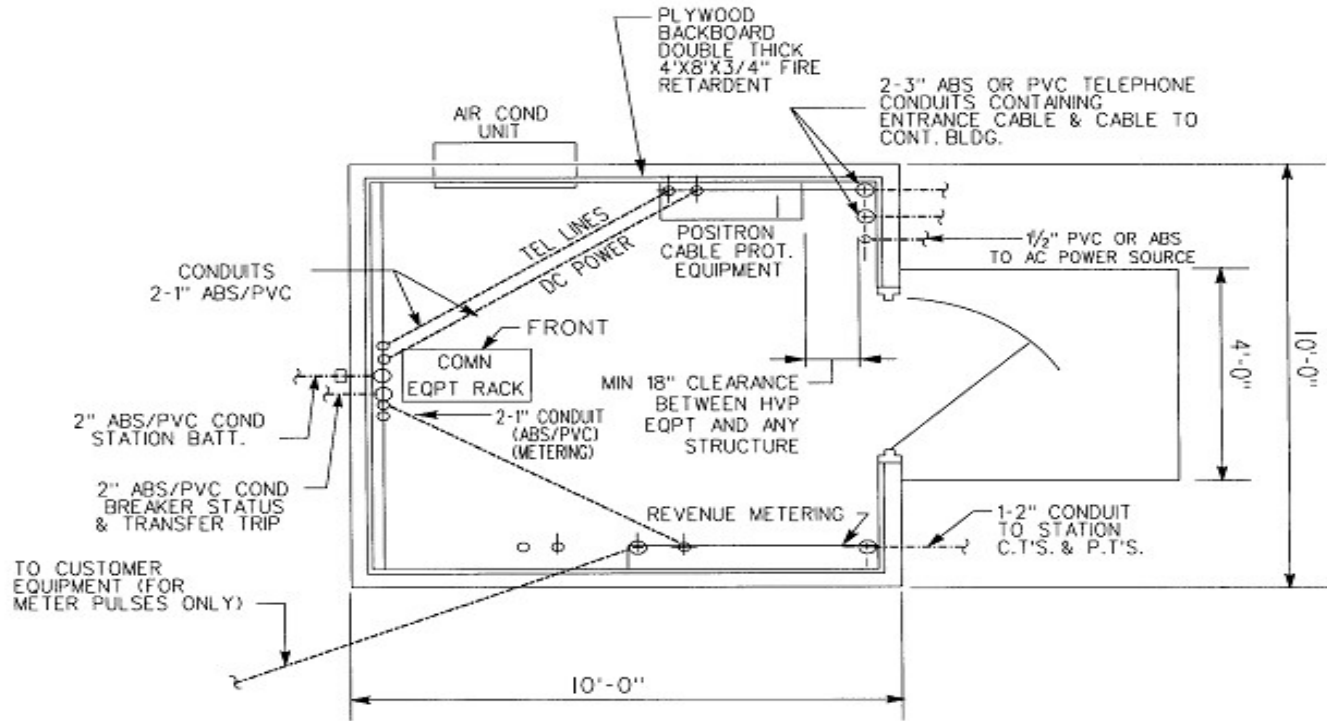
FIGURE F-4 SUGGESTED ROOM LAYOUT FOR SMALL GENERATORS
