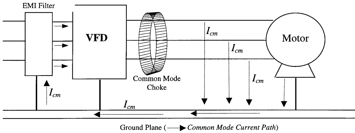
Figure 3 – Mitigating common mode effects by impeding flow of common mode currents with a Common Mode Choke or by providing low-impedance path with an EMI Filter.
